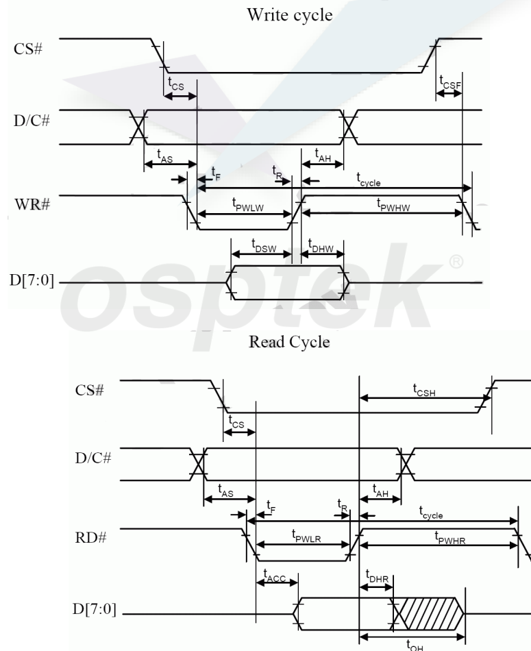
8080-series parallel interface characteristics
