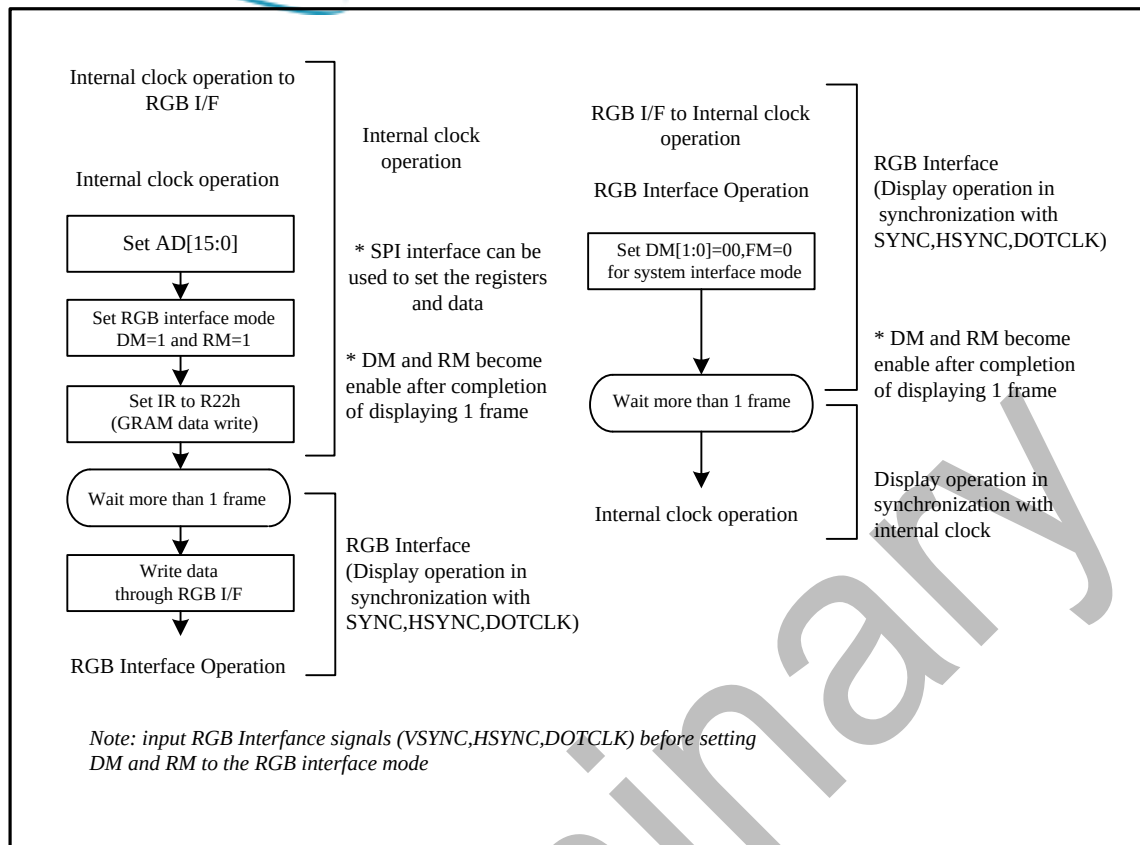
Figure15 Internal clock operation/RGB interface mode switching
