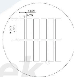
Detail A 500:1
